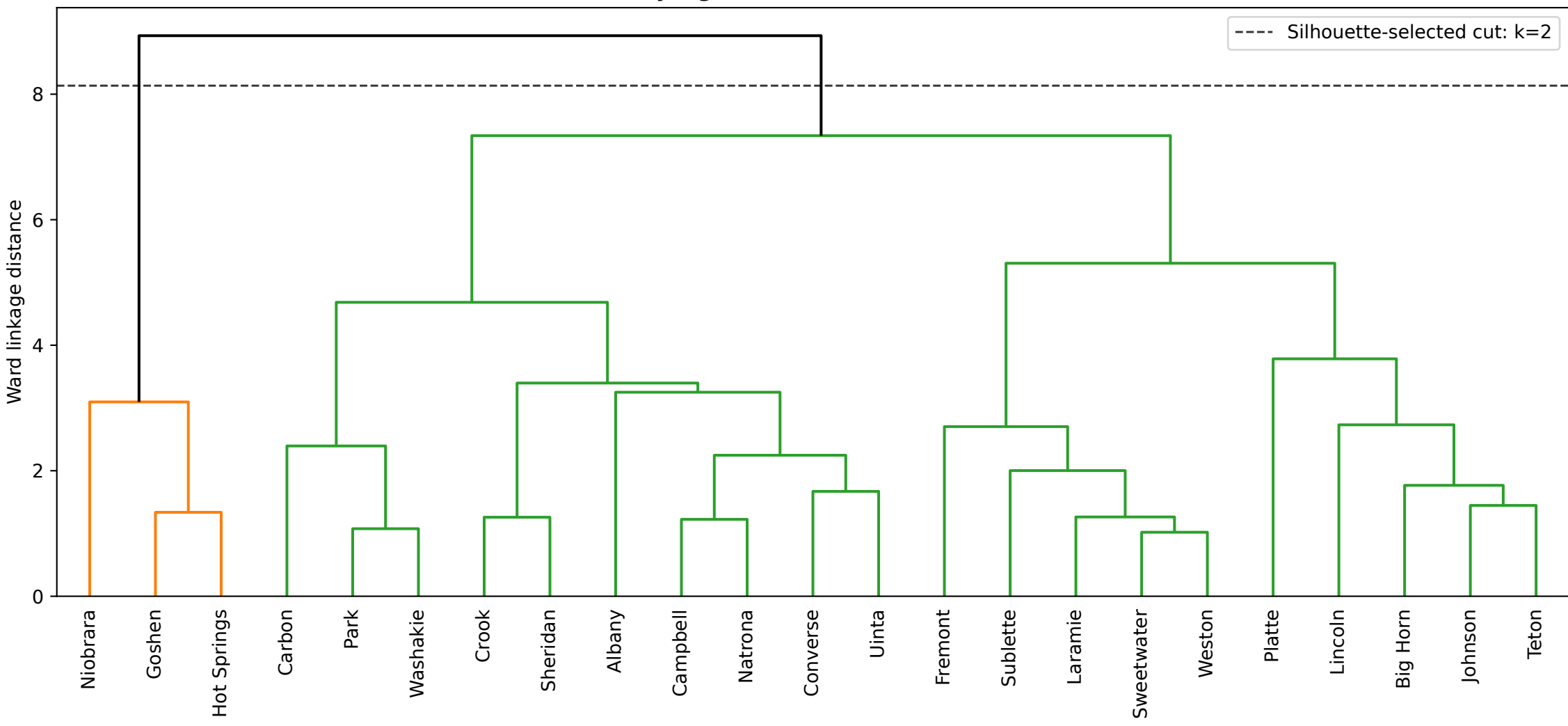
Ward Dendrogram — Simplified 6-Feature Space, 14-day Sakoe-Chiba Band Branch colors forced by highest silhouette score: k=2, silhouette=0.359
